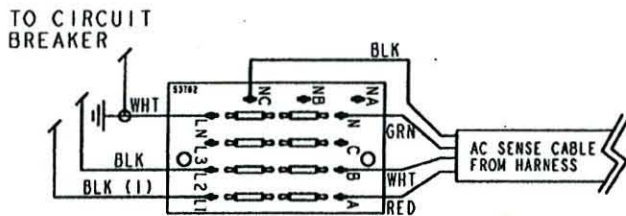
VOLTAGE SENSE RESISTOR BOARD PN#053762 (NEW)
